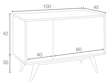
01 VINTAGE - Puerta, cajón - Porte, tiroir - Door, drawer
