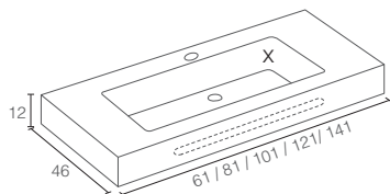
FRONTE HERO SOLID SURFACE
