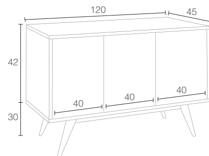
01 VINTAGE - Puerta, cajón, puerta - Porte, tiroir, porte - Door, drawer, door
